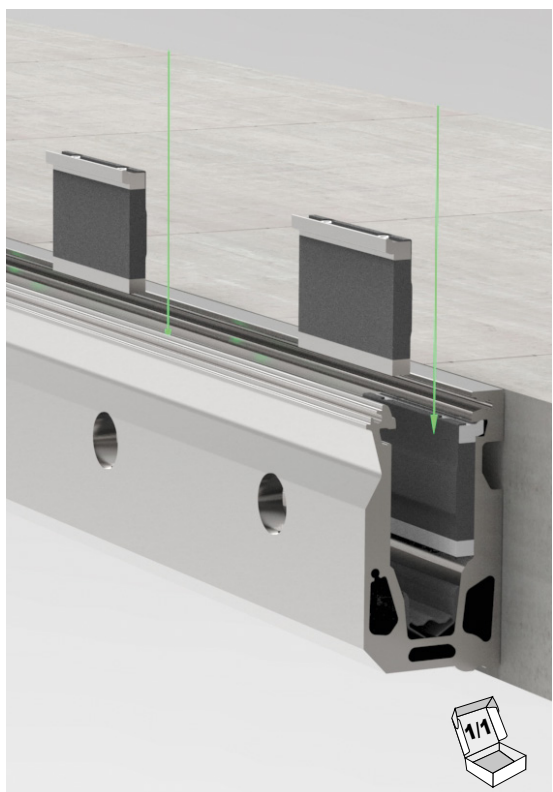
Klemmsystem | clamp system
